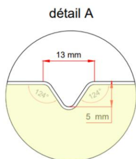
Figure 2 – Panneau sandwich isolant Evolution Multi Groove
