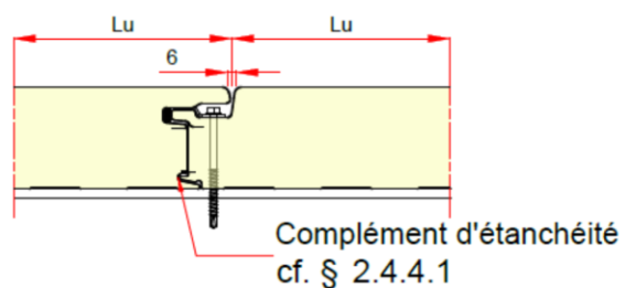
Figure 2 – Panneau sandwich isolant Evolution Multi Groove
