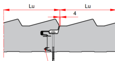
Figure 3 – Panneau sandwich isolant Louvre
