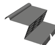
1/2 toothed ridge adaptable to the slope with ventilated flange
