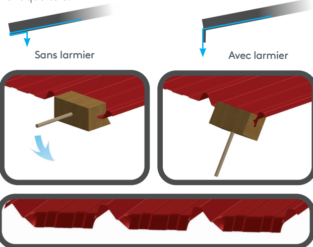
Larmier
