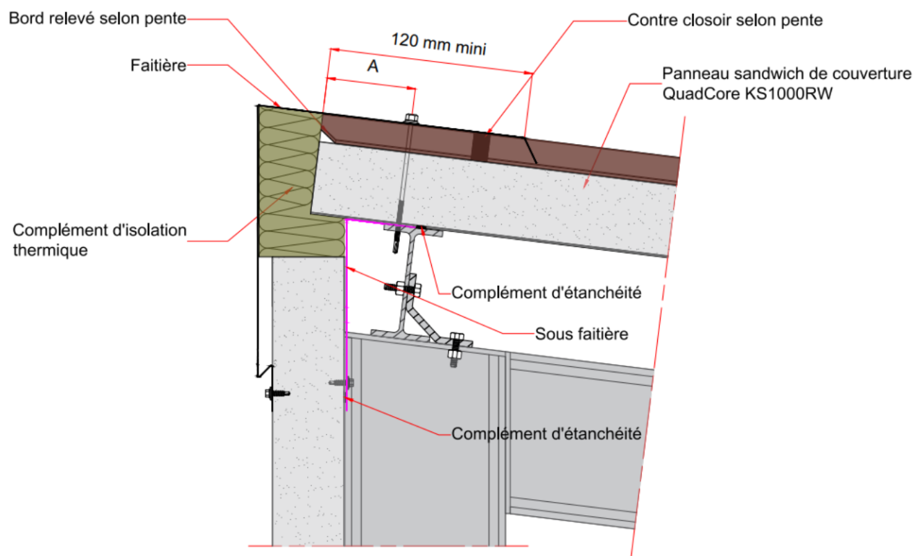
Figure 8 – Faitage simple
