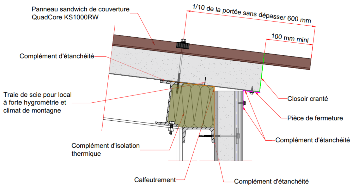
Figure 12 – Egout sans gouttière
