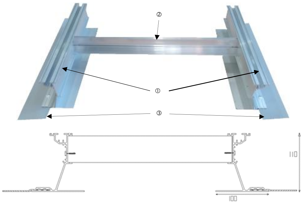
Figure 2 - Ossature Support iNova PV Lite
