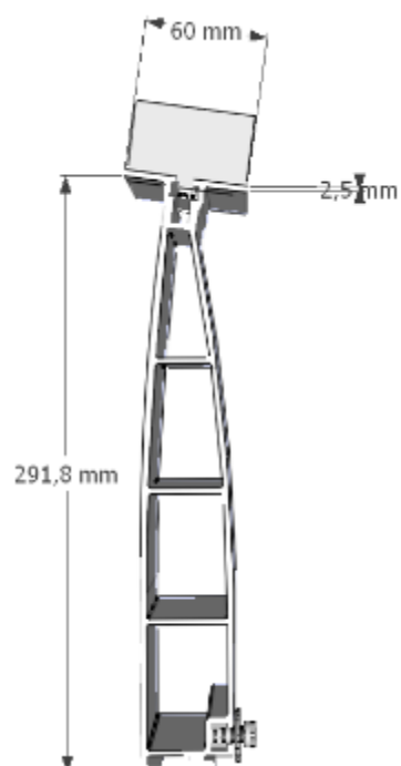
Figure 8 – Rehausse Tilt GC FE haute de 8°
