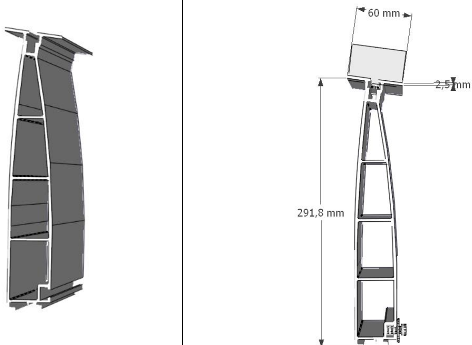
Figure 8 – Rehausse Tilt GC FE haute de 8°
