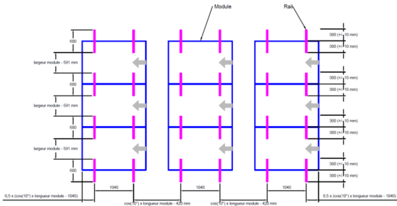
Figure 35 - Implantation des rails / modules simple shed
